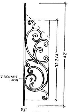
D-3 TOP VIEW ALL RADIUS FROM 30" TO 20'-0"
