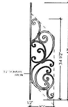
PIECE E FITS ANGLES 37° TO 48°
