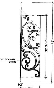
D-2 TOP VIEW ALL RADIUS FROM 30" TO 20'-0"
