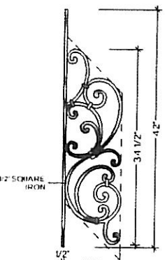
E-3 TOP VIEW ALL RADIUS FROM 30" TO 20'-0"
