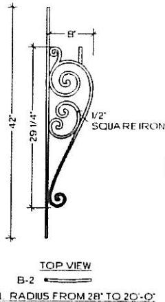
ALL RADIUS FROM 28" TO 20'-0"
