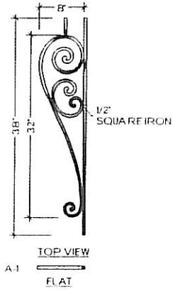
PIECE A FITS LEVEL BALCONY OR STRAIGHT RAILS
