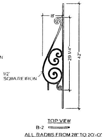
ALL RADIUS FROM 28" TO 20'-0"
