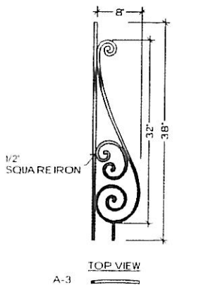
ALL RADIUS FROM 28" TO 20'-0"
