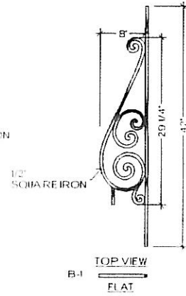
PIECE B FITS ANGLES UP TO 48°
