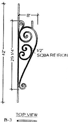
ALL RADIUS FROM 28" TO 20'-0"
