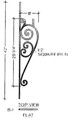
PIECE B FITS ANGLES UP TO 48°
